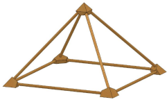
Pyramide
